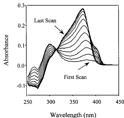
FIGURE 2: Time-resolved UV difference spectra of D145N (25 \mu M) with 4-CBA-CoA (25 \mu M) in 50 mM K^+ Hepes (pH 7.5, 25 ^{\circ}\text{C} ): 6 s per scan with 30 s delay between scans.
