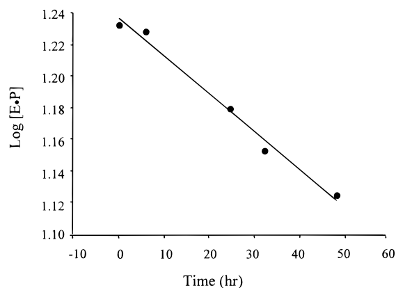
FIGURE 1: Time course of the "spontaneous" deamidation of D145N (19 \mu M) in 50 mM K^+ Hepes, pH 7.5, at room temperature in the absence of 4-HBA-CoA.
